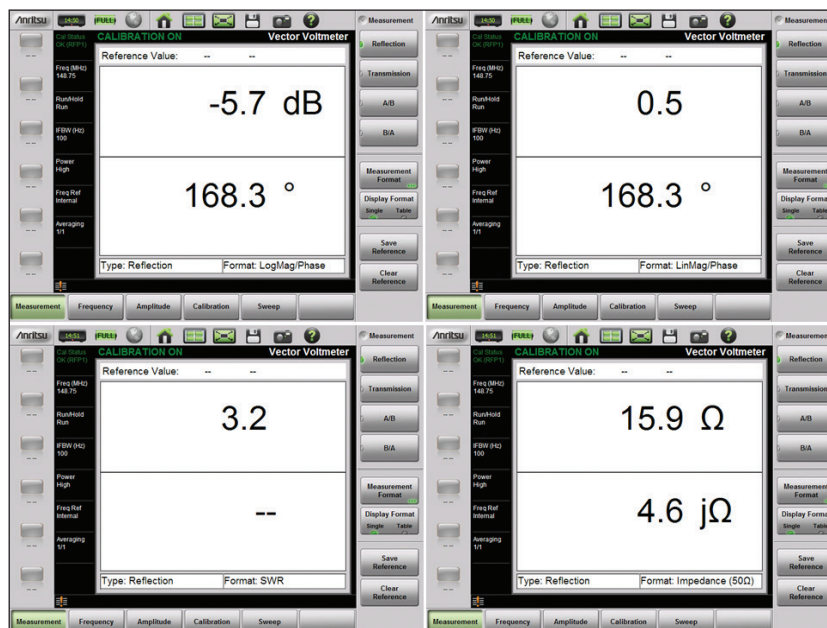
Select Which Data Display Format You Prefer, the Site Master S820E Converts the Format Automatically for You
