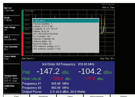
Test Reports generated using Line Sweep Tools (LST)
